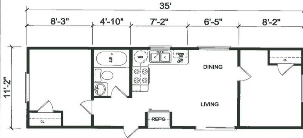
Model 143 - 399 Square Feet
